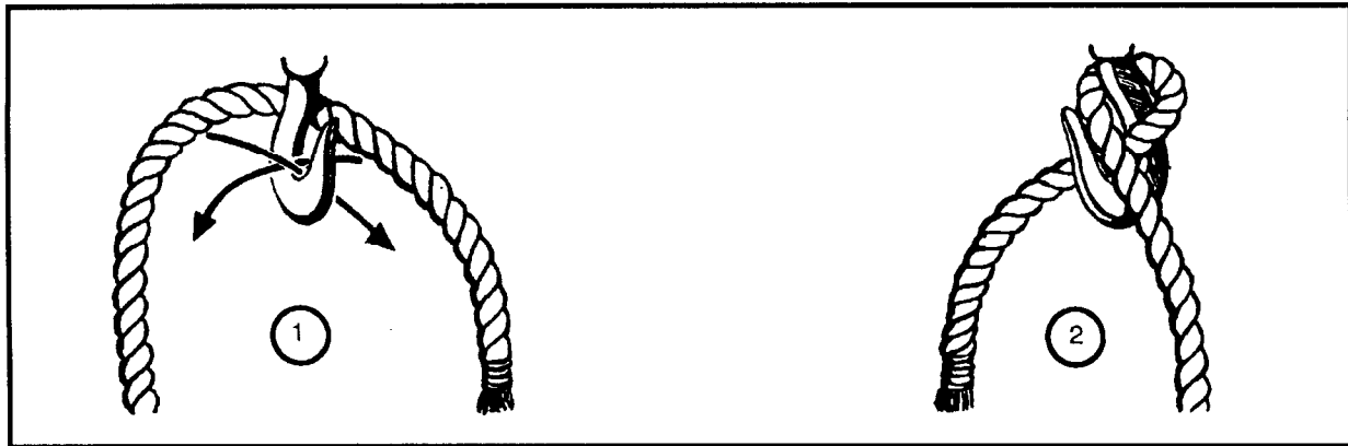
Figure 2-31. Blackwall hitch
