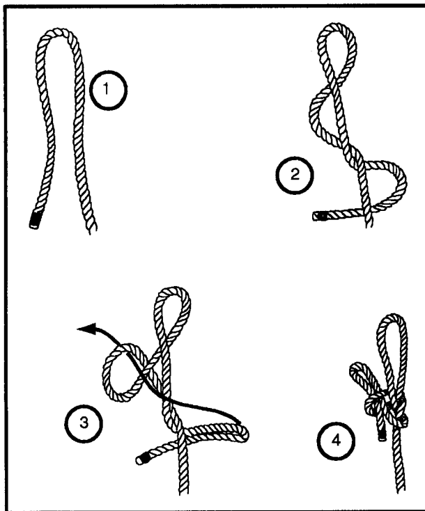
Figure 2-17. Speir knot
