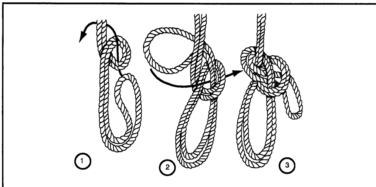
Figure 2-12. Double bowline
