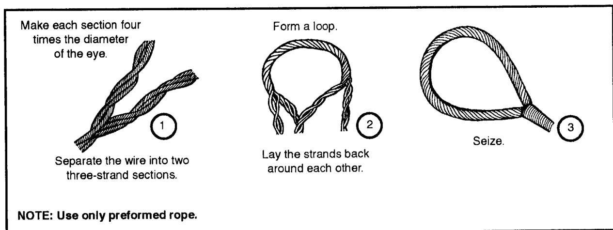
Figure 2-47. Hasty eye splice for wire rope
