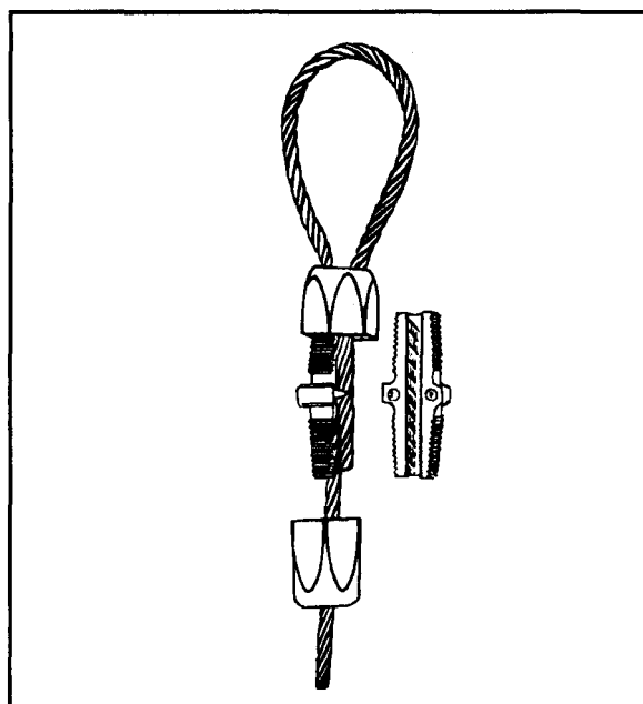
Figure 2-51. Wire-rope clamps
