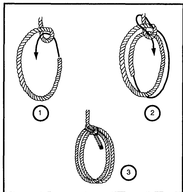
Figure 2-16. French bowline
