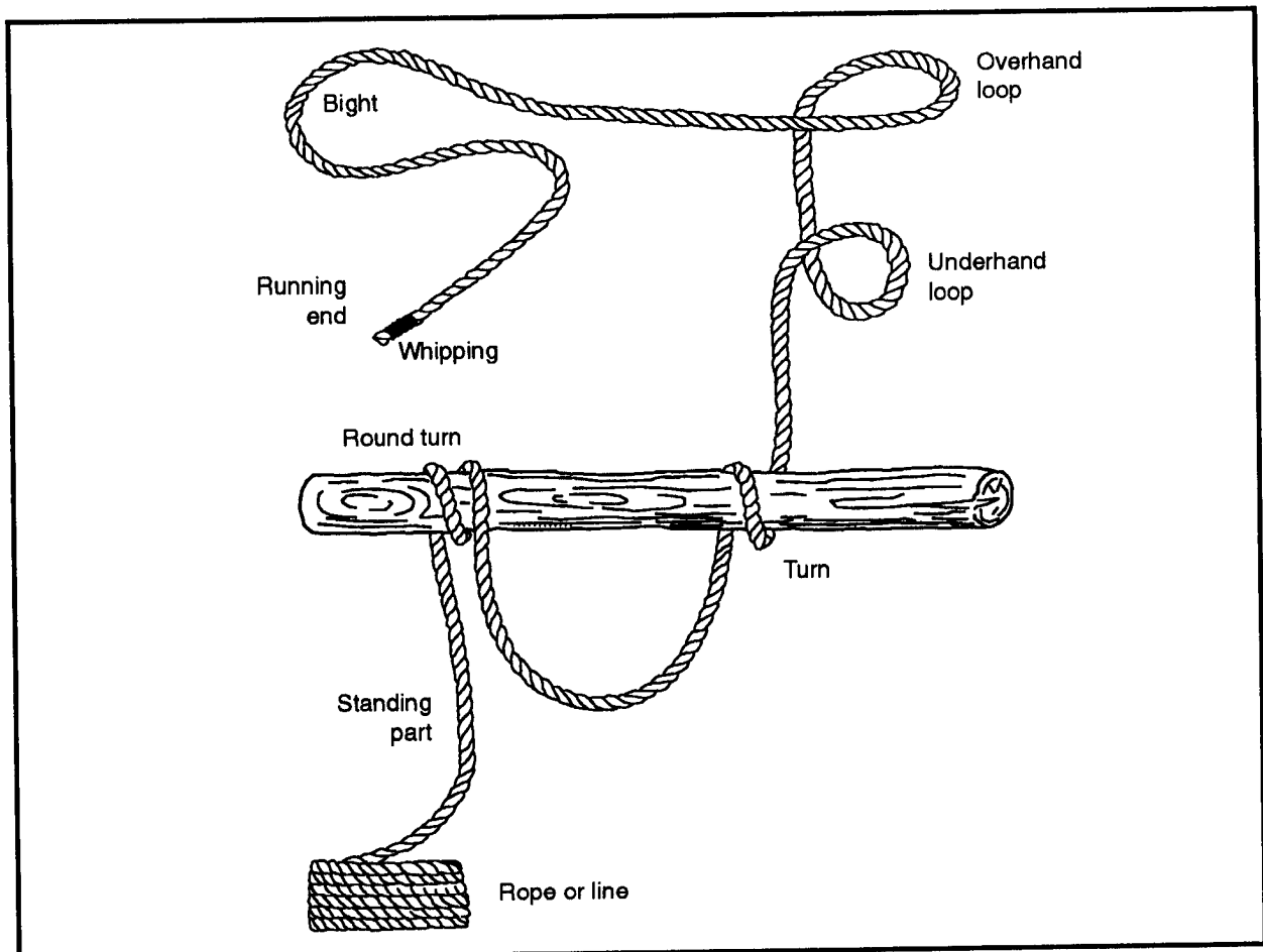
Figure 2-1. Elements of knots, bends, and hitches
