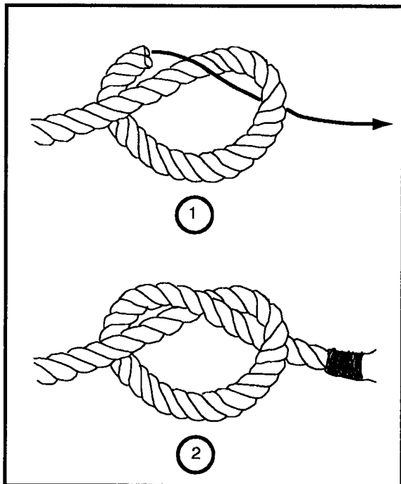
Figure 2-3. Overhand knot
