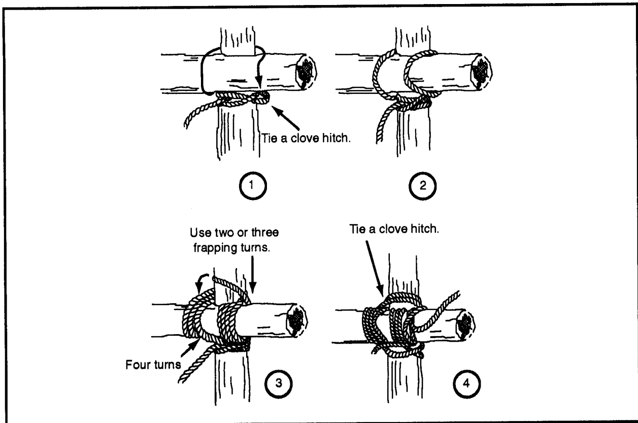
Figure 2-36. Square lashing
