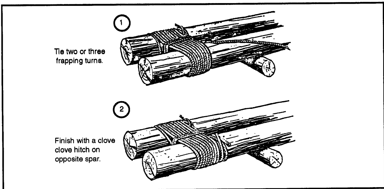
Figure 2-37. Shears lashing
