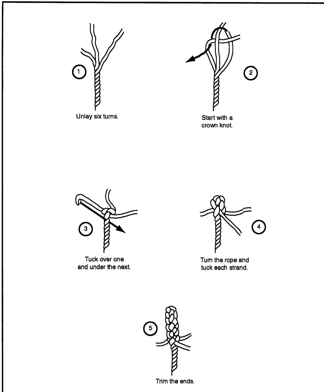
Figure 2-43. Crown or back splice for fiber rope
