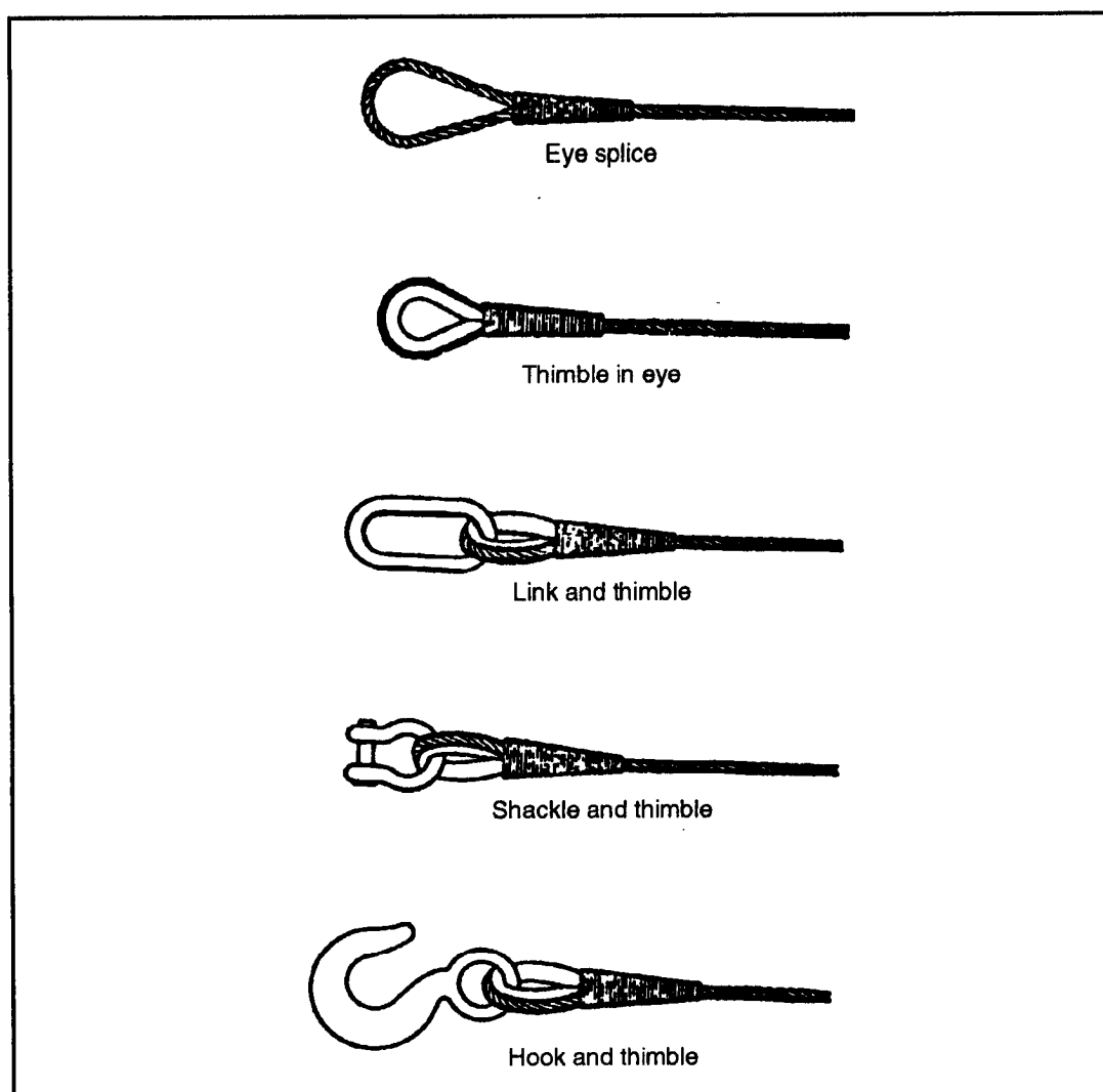
Figure 2-49. Attachments used with eye splice
