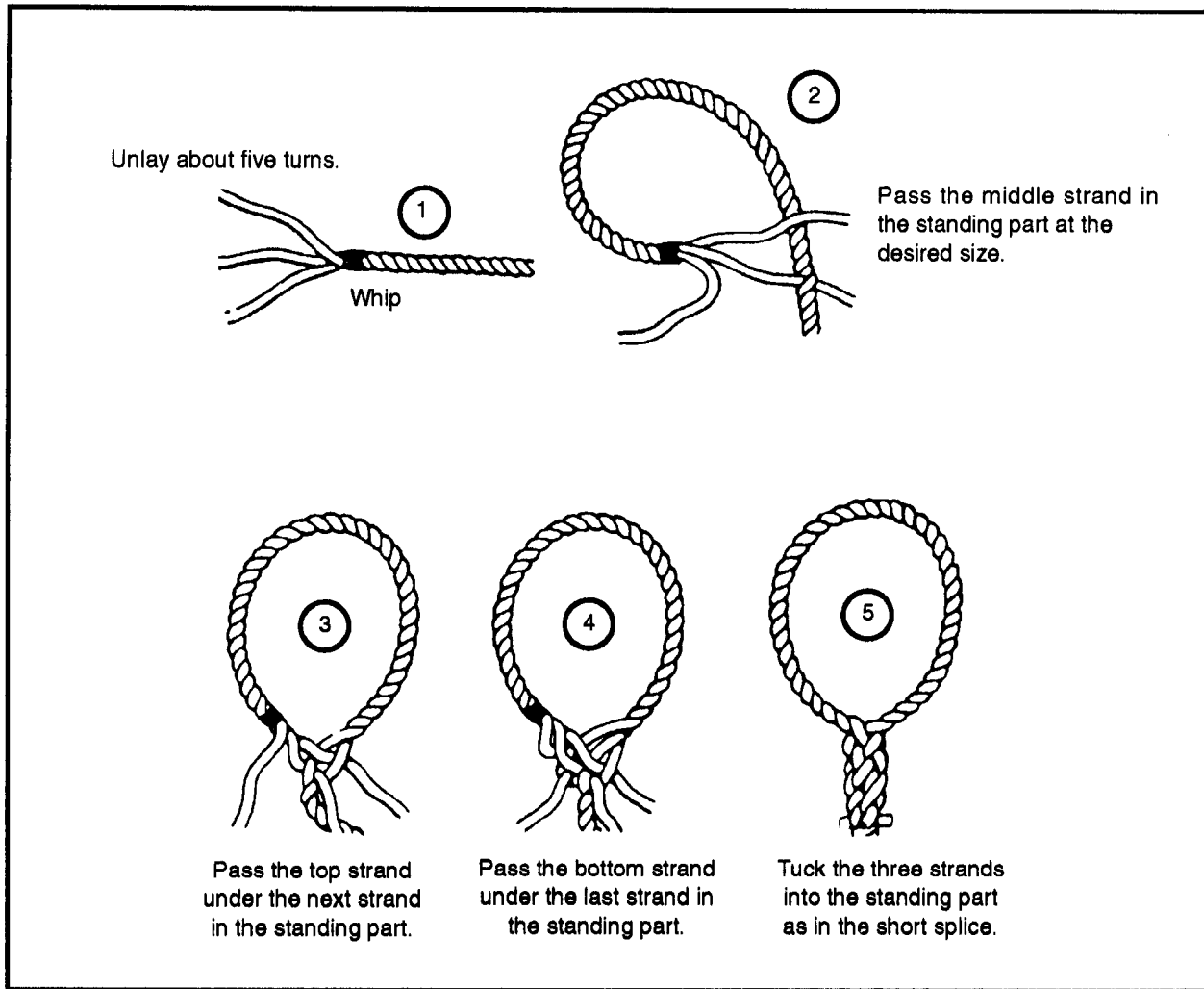
Figure 2-41. Eye or side splice for fiber rope
