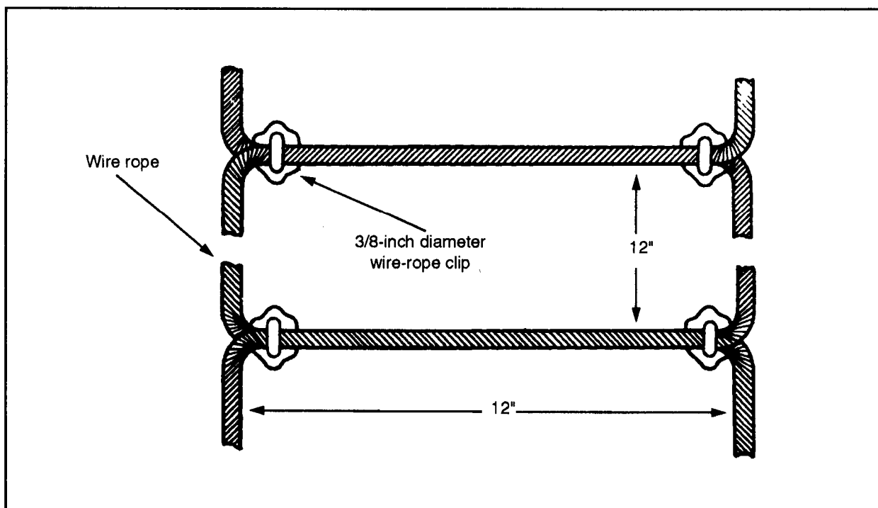
Figure 2-58. Wire-rope rungs
