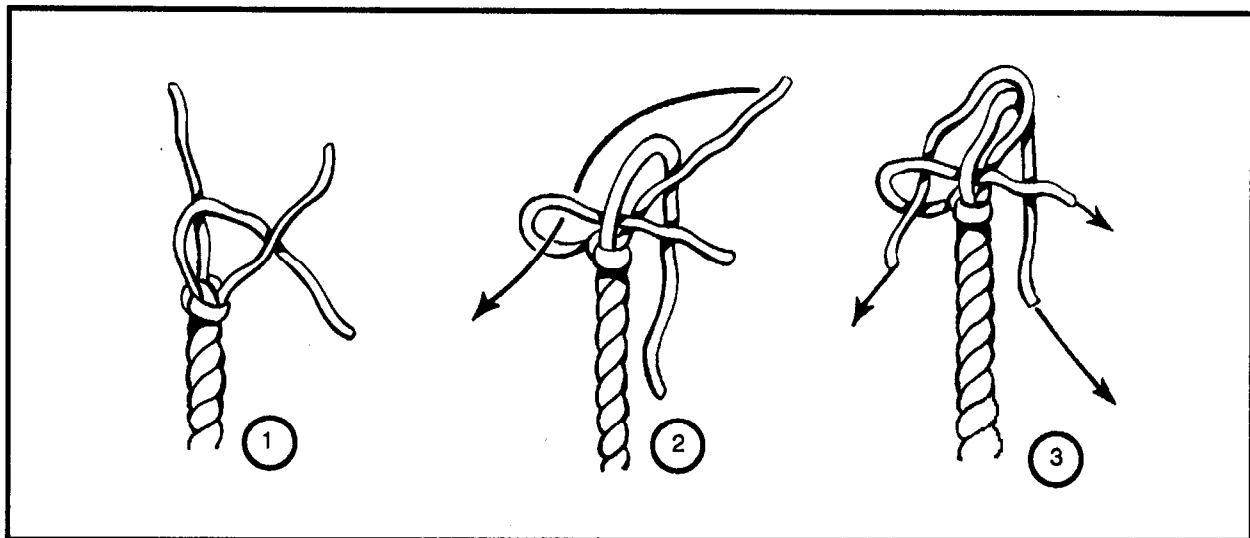
Figure 2-6. Crown on a wall knot
