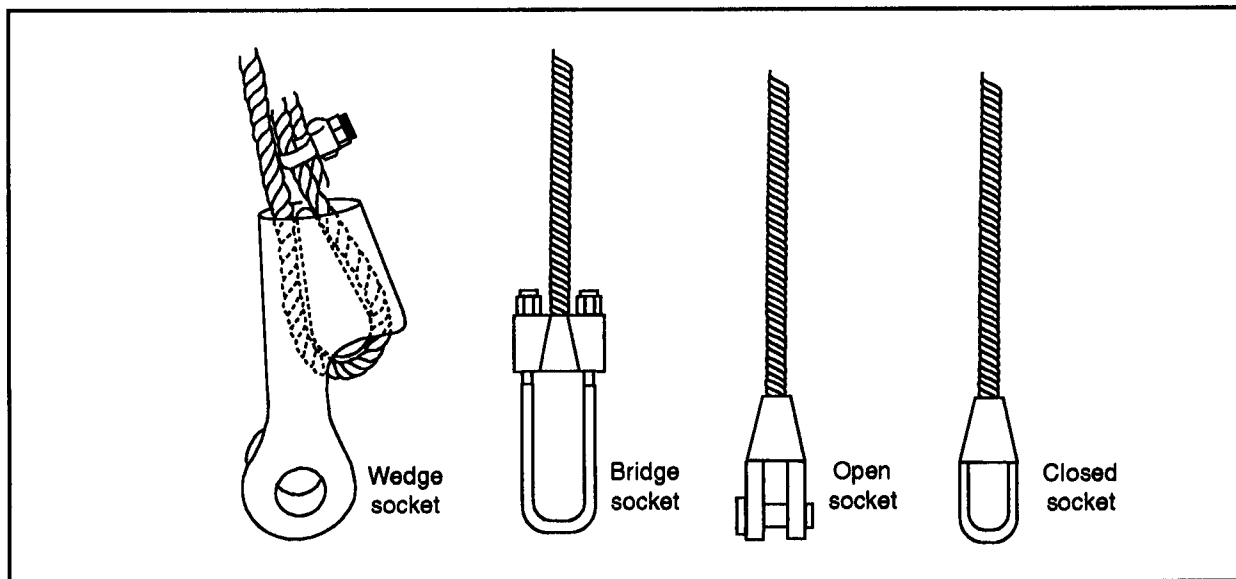
Figure 2-53. Basket-socket end fittings
