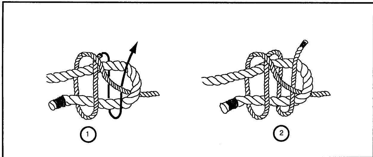
Figure 2-9. Double sheet bend
