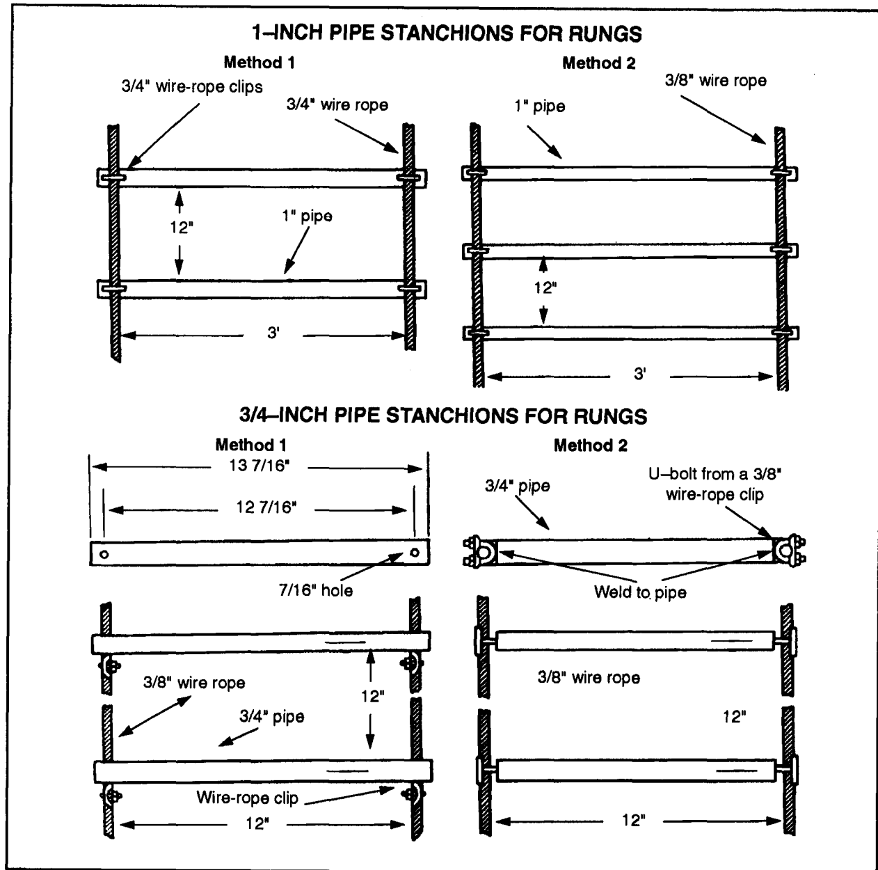
Figure 2-57. Pipe rungs
