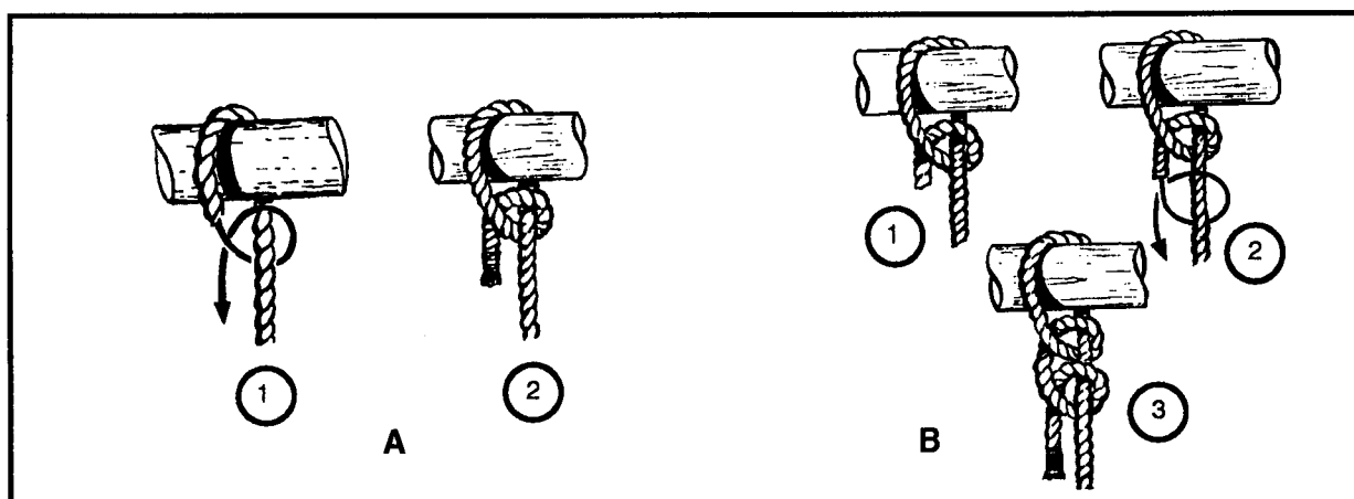
Figure 2-22. Half hitches
