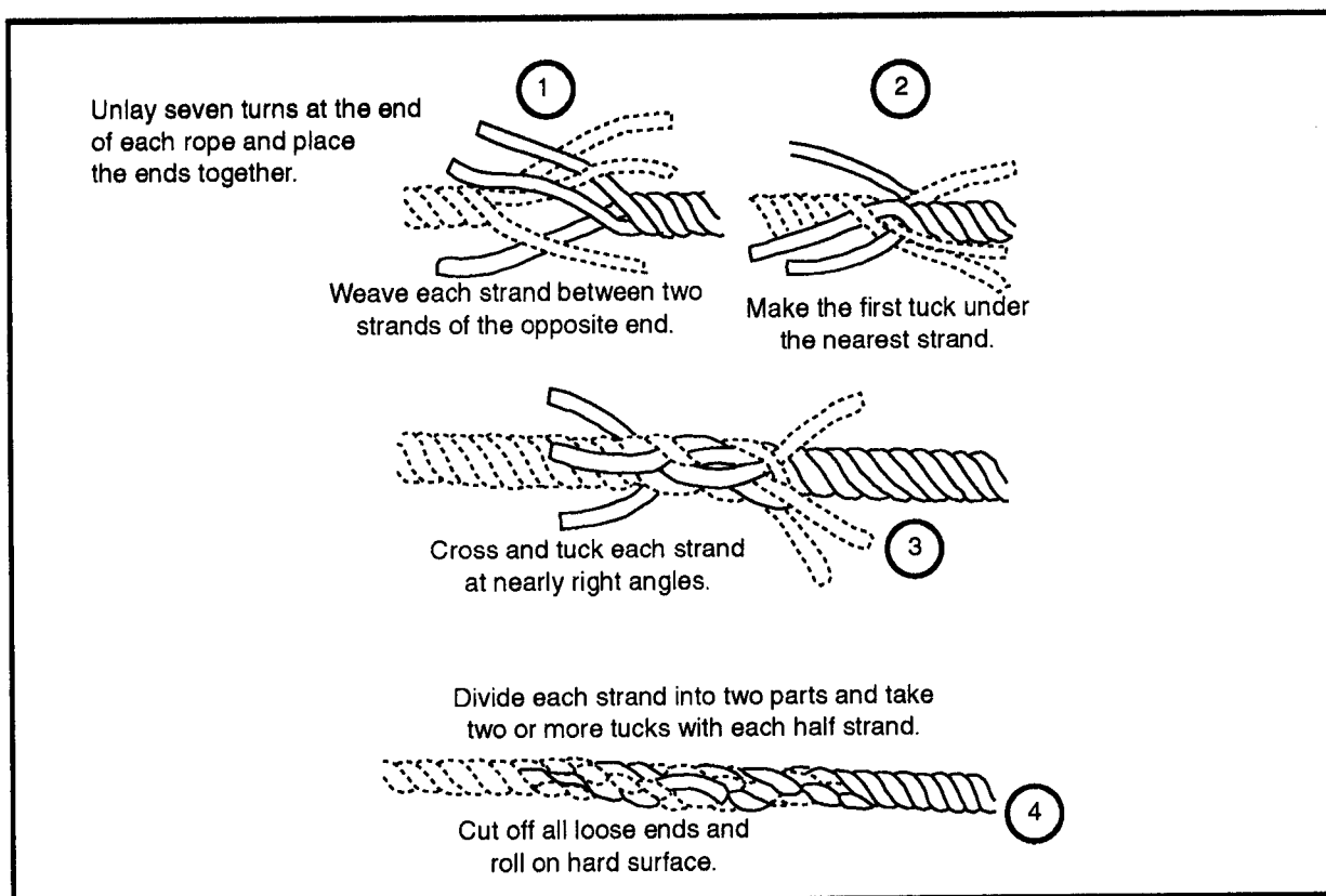
Figure 2-40. Short splice for fiber rope
