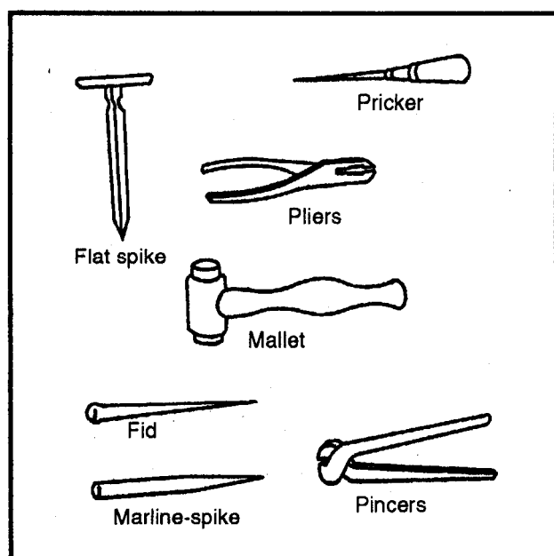
Figure 2-44. Tools for wire splicing
