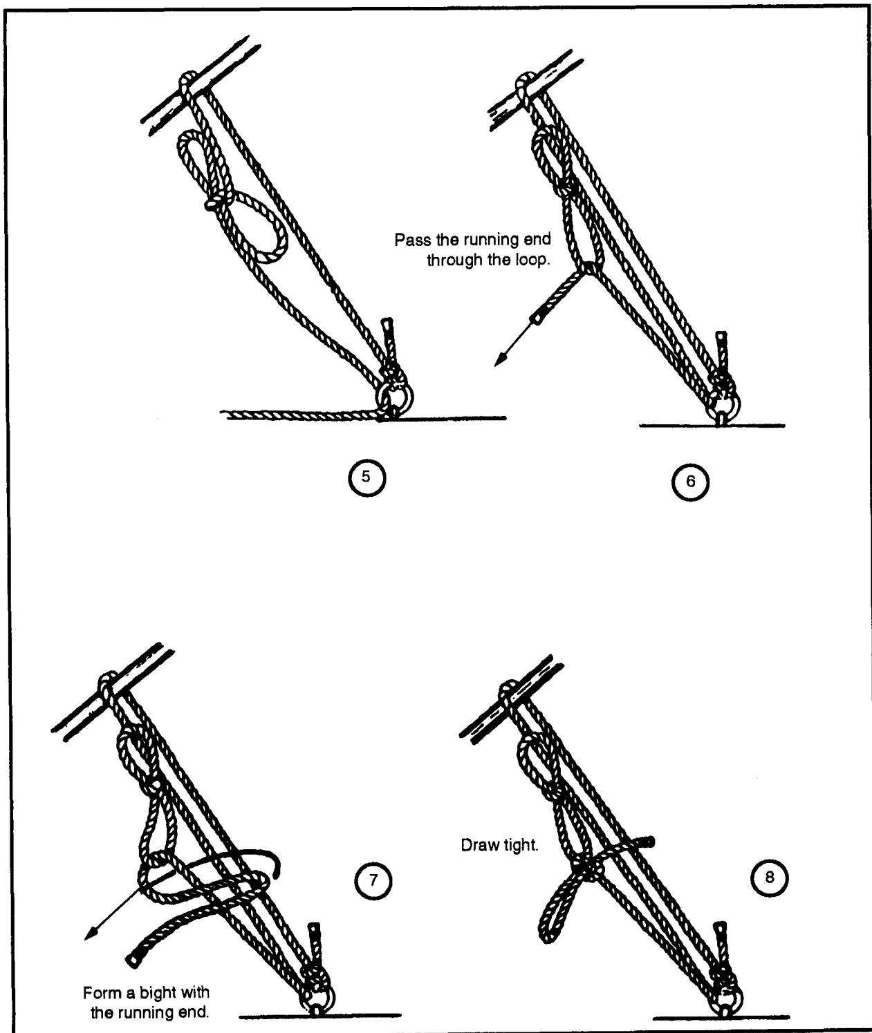
Figure 2-21. Baker bowline (continued)
