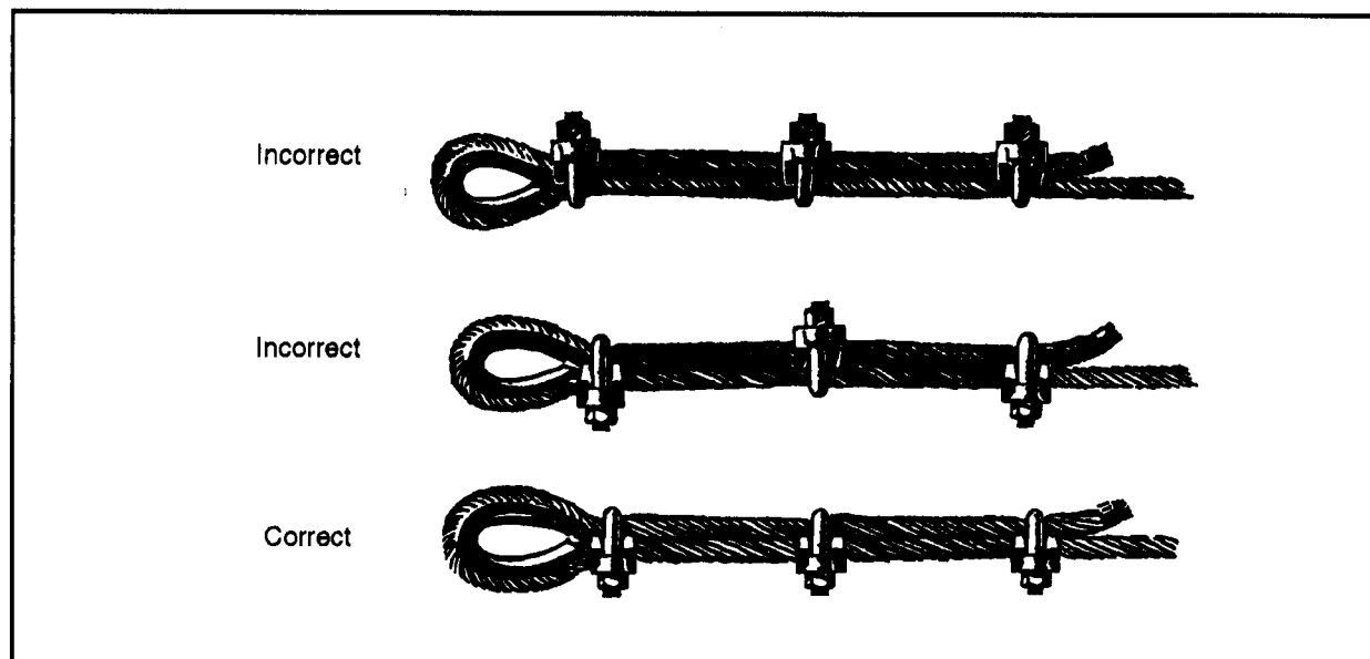
Figure 2-50. Wire-rope clips
