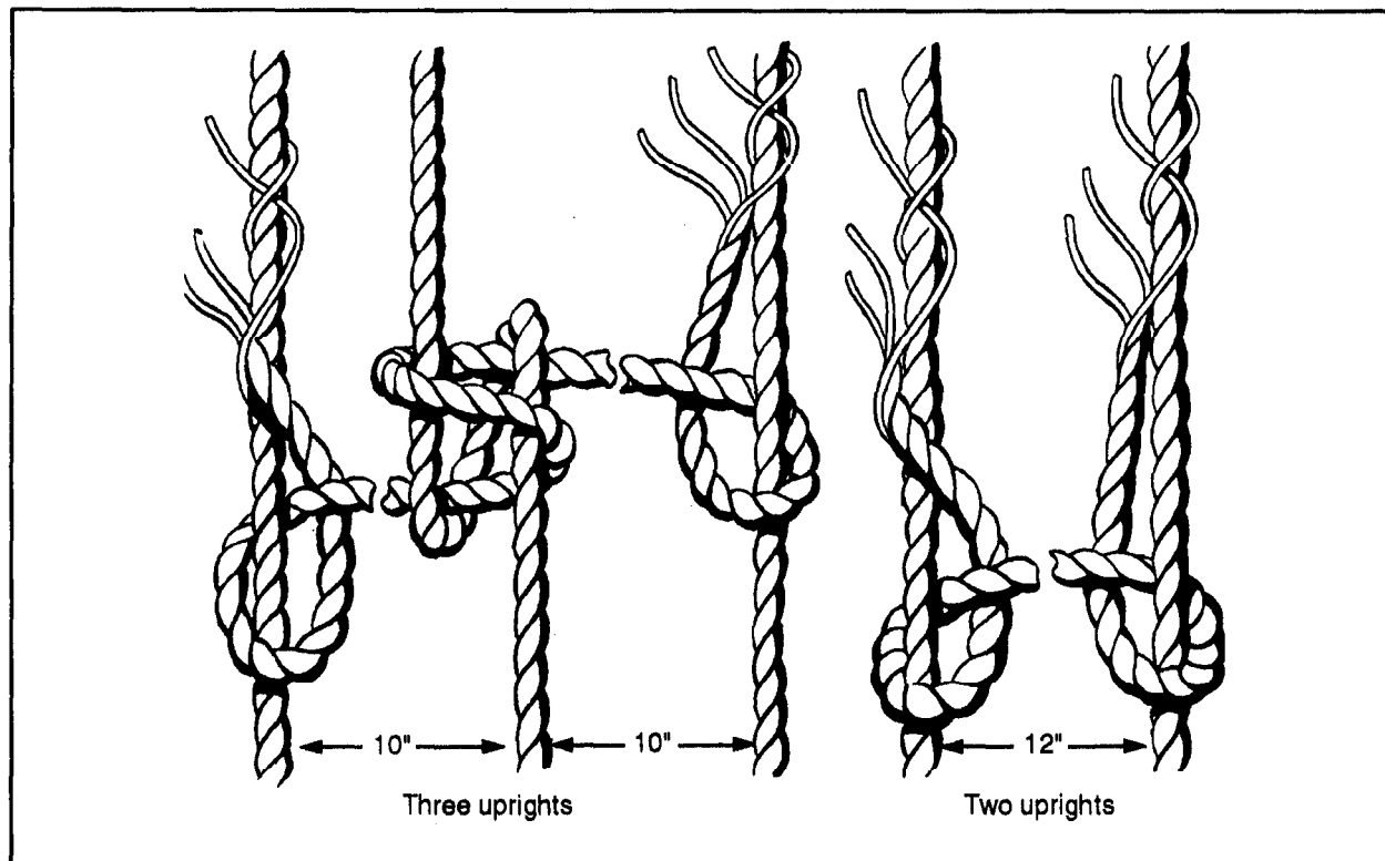
Figure 2-59. Fiber-rope rungs
