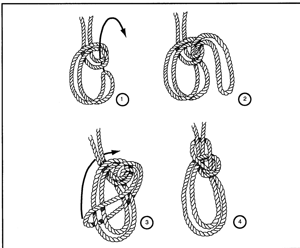
Figure 2-14. Bowline on a bight
