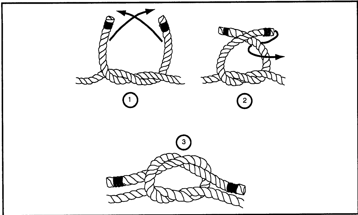
Figure 2-7. Square knot
