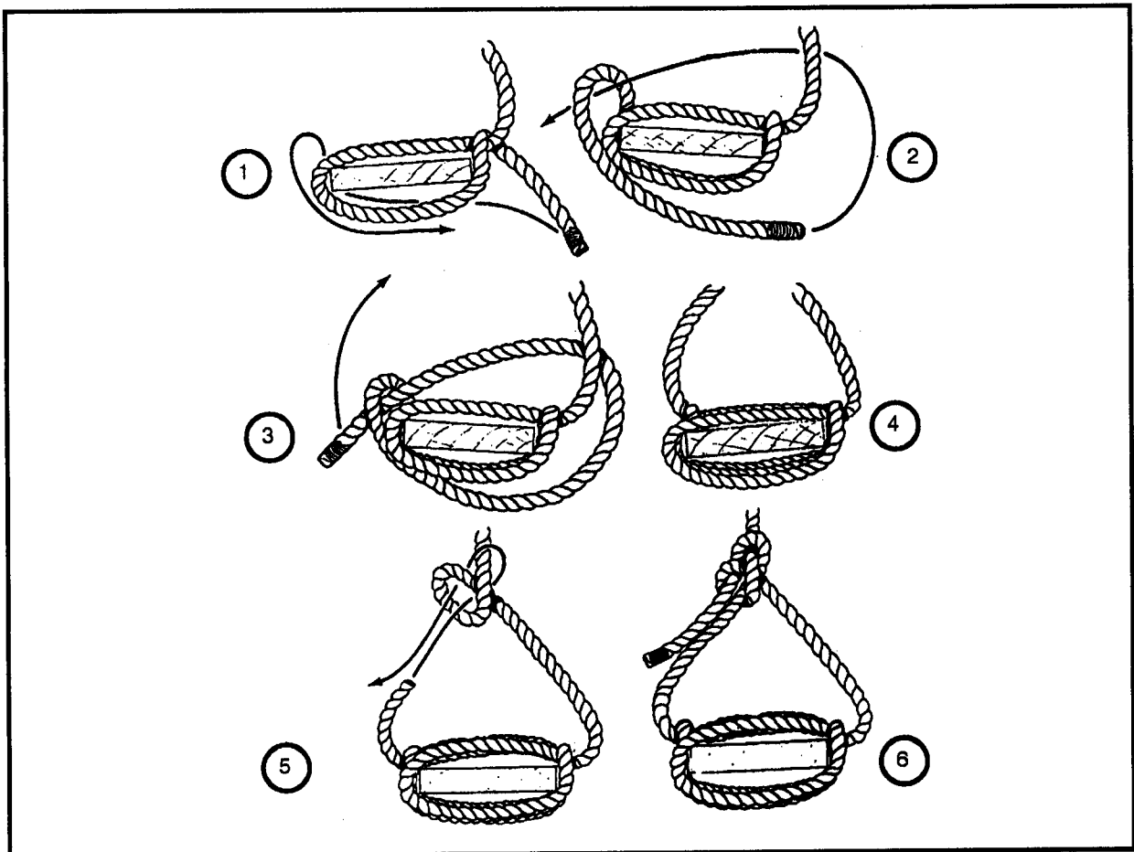
Figure 2-30. Scaffold hitch
