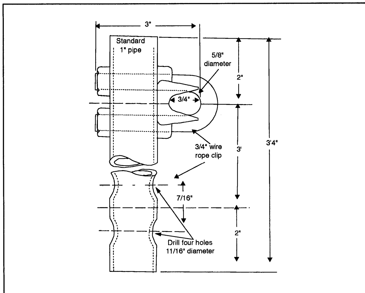
Figure 2-56. Iron-pipe stanchions
