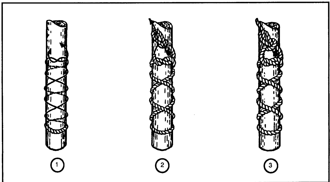
Figure 2-28. Telegraph hitch
