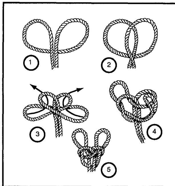
Figure 2-15. Spanish bowline
