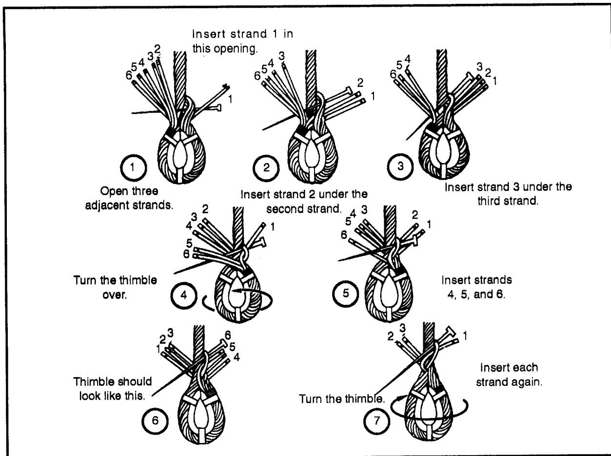
Figure 2-46. Eye splice with thimble for wire rope
