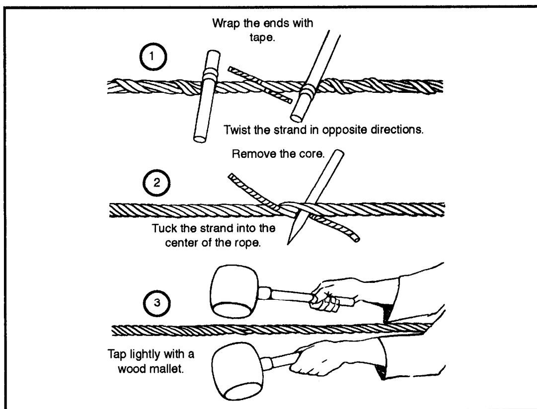
Figure 2-45. Tucking wire-rope strands
