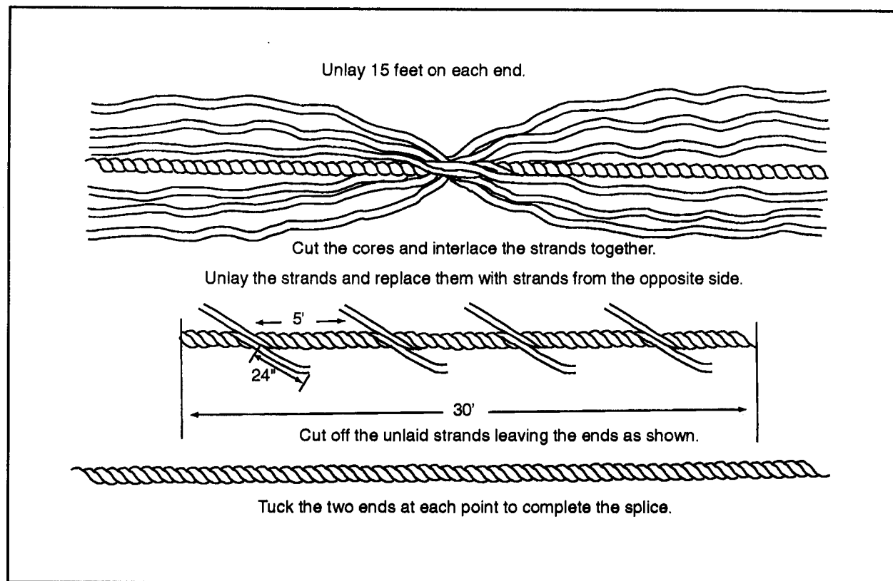
Figure 2-48. Long splice for wire rope
