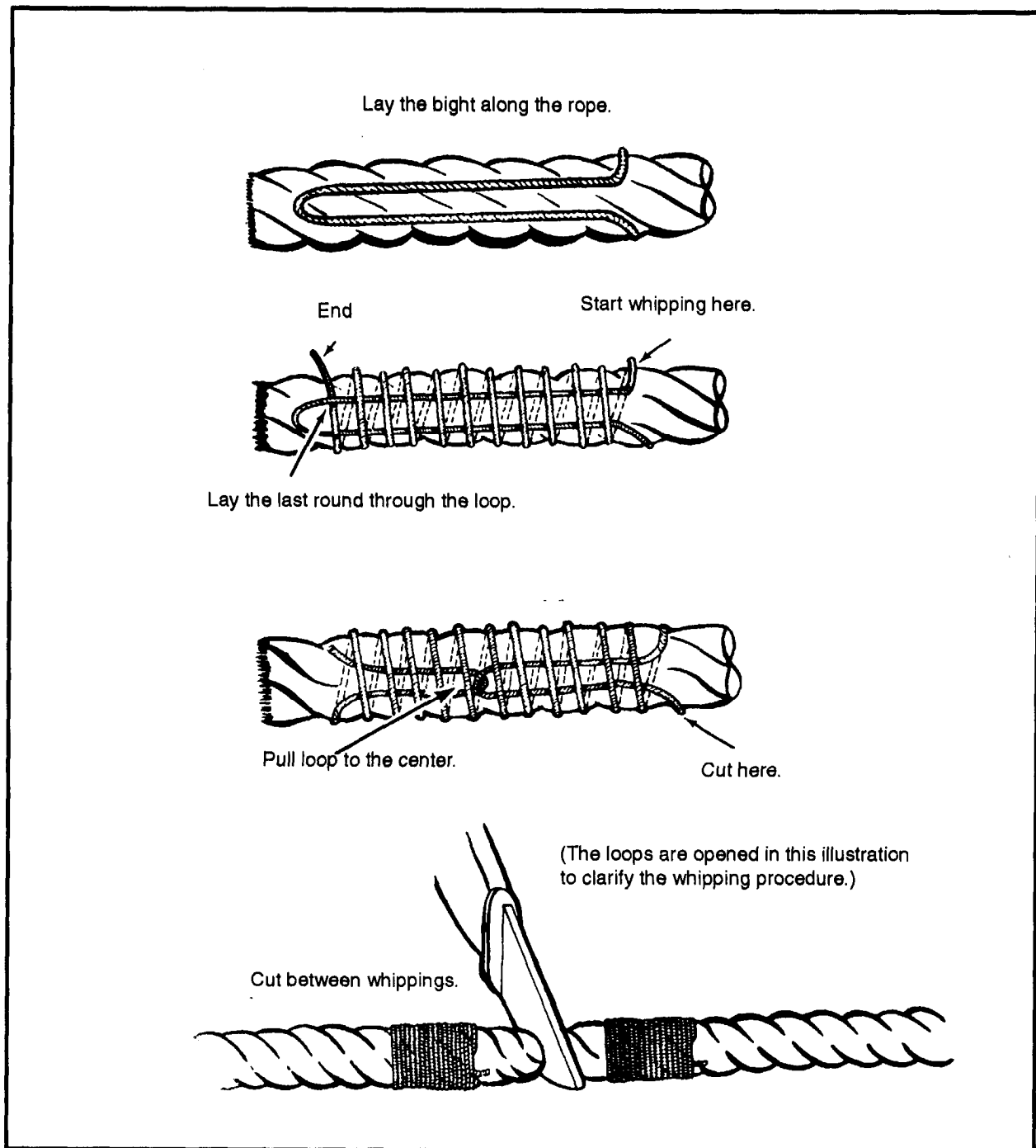
Figure 2-2. Whipping the end of a rope
