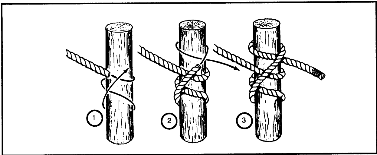
Figure 2-29. Mooring hitch
