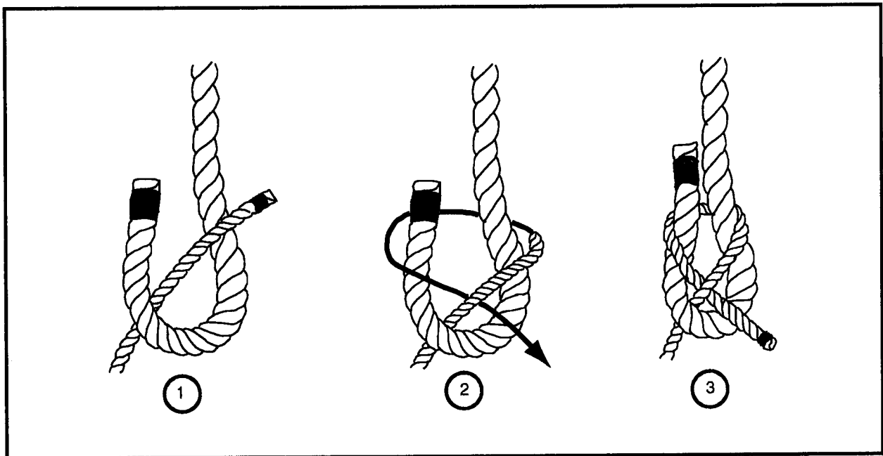
Figure 2-8. Single sheet bend
