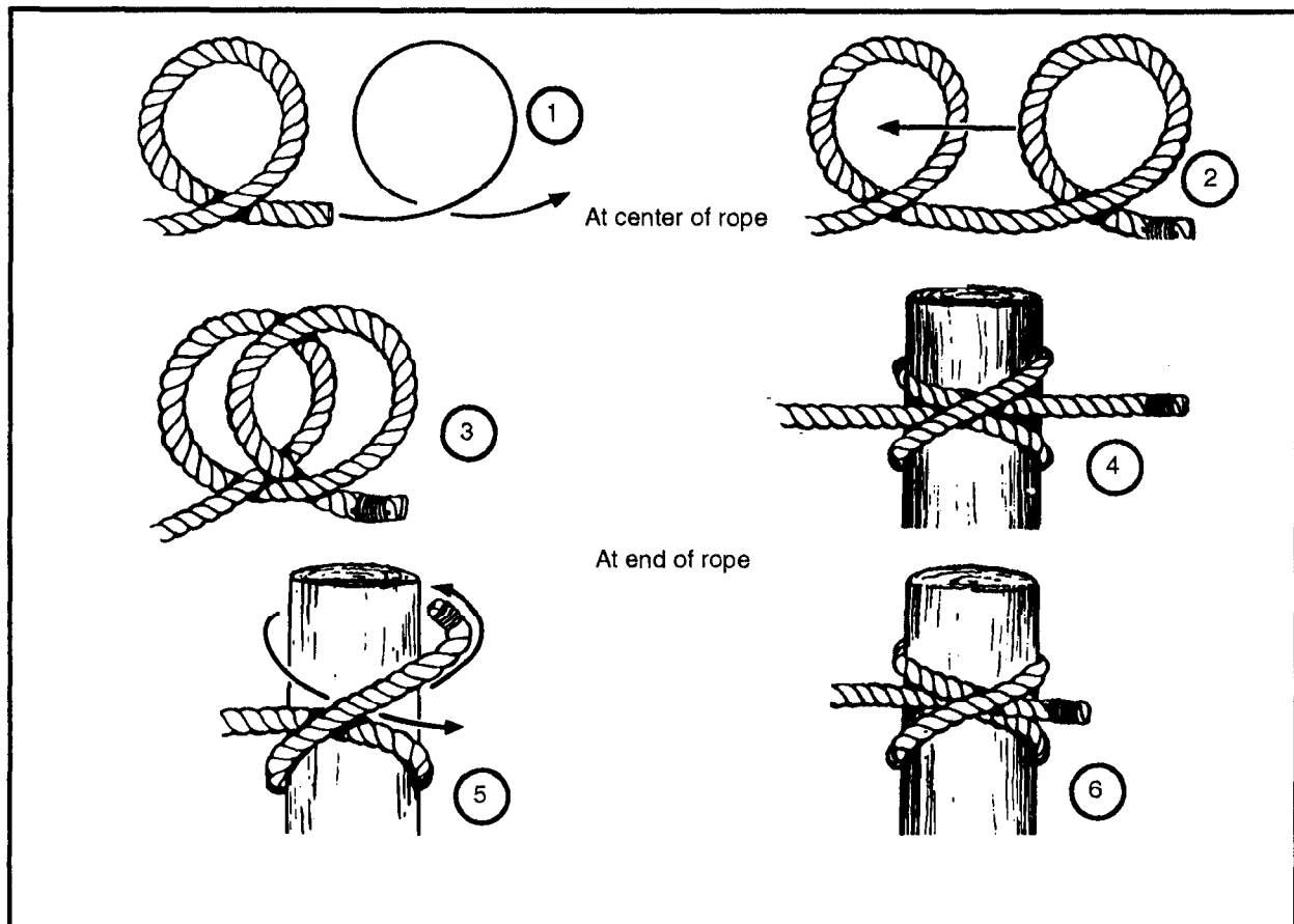
Figure 2-26. Clove hitch
