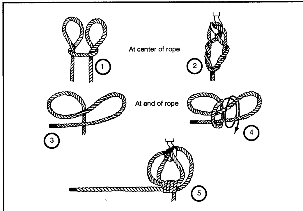
Figure 2-18. Cats-paw
