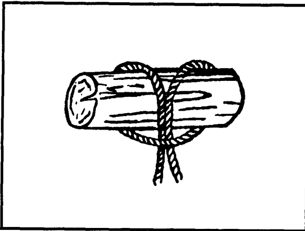
Figure 2-33. Girth hitch
