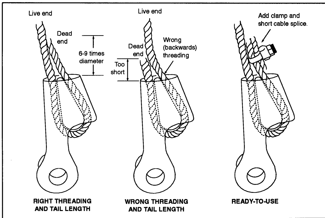
Figure 2-52. Wedge socket
