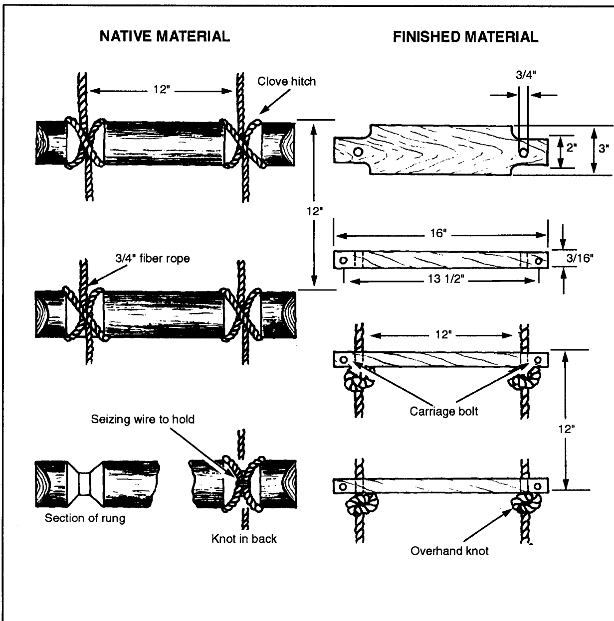
Figure 2-60. Wood rungs
