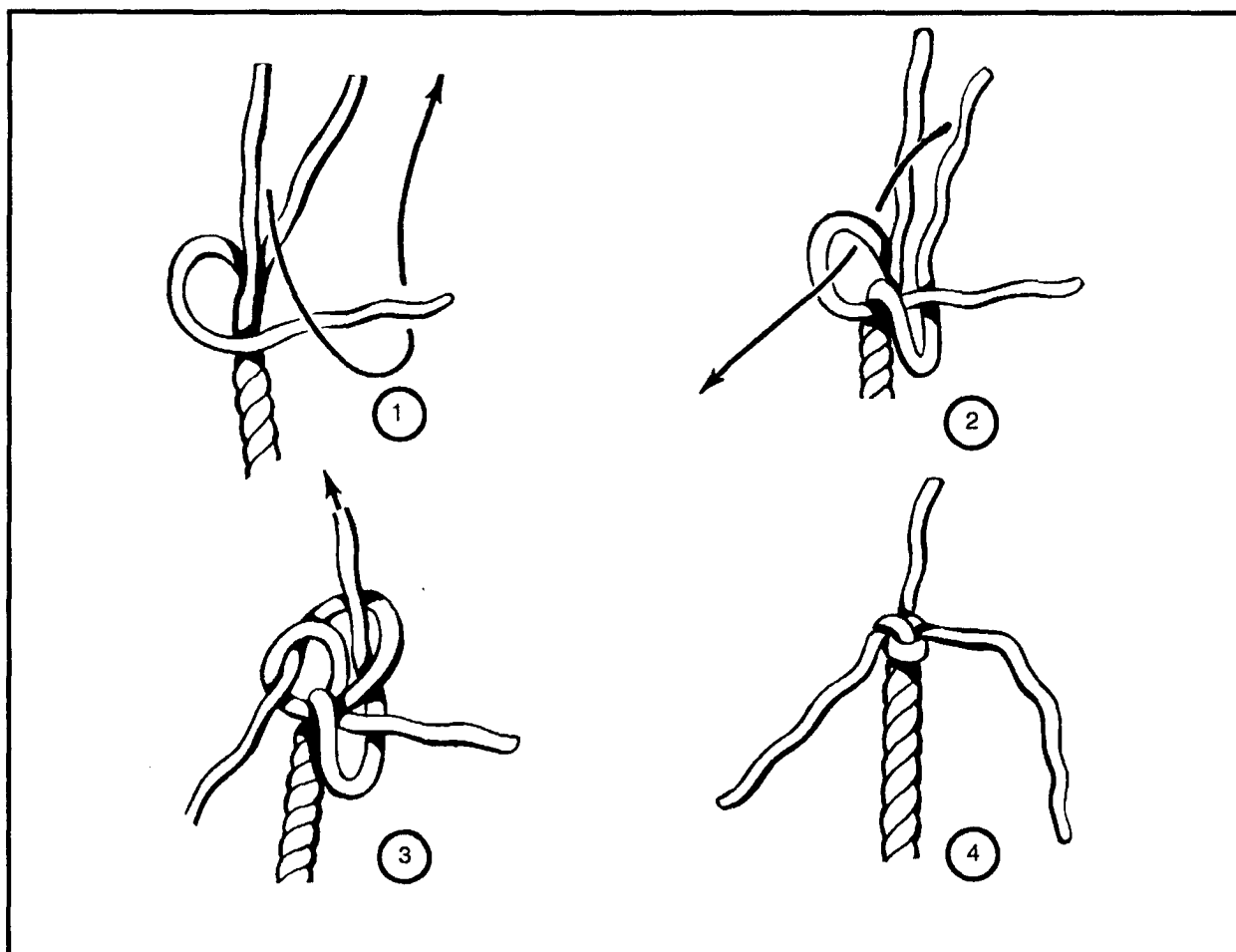
Figure 2-5. Wall knot
