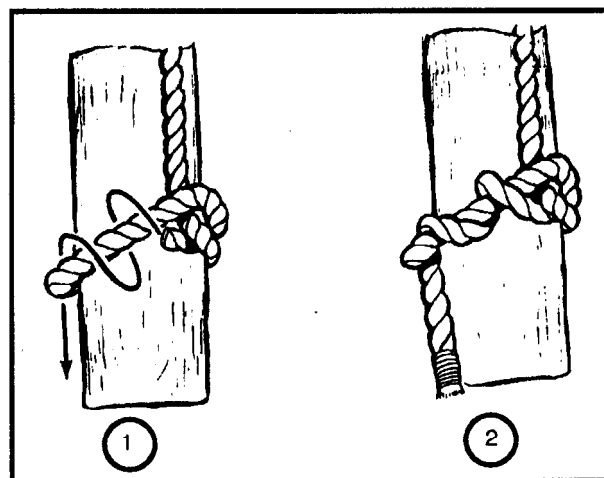
Figure 2-24. Timber hitch
