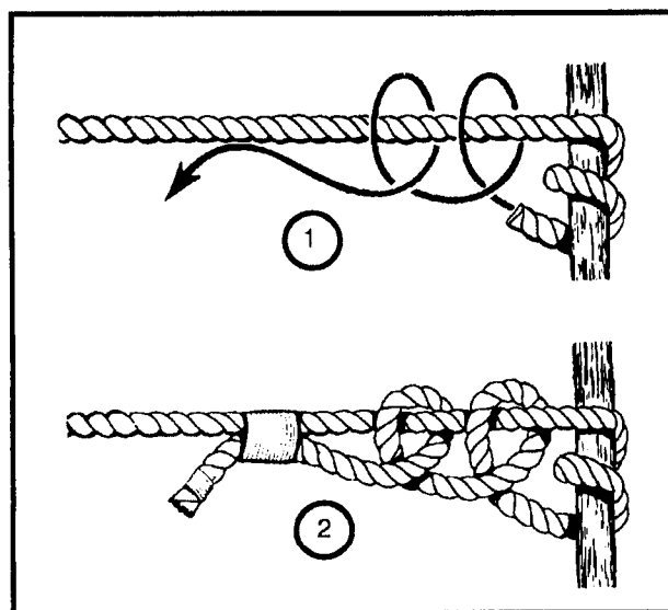
Figure 2-23. Round turn and two half hitches
