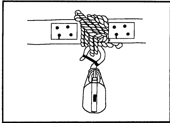
Figure 2-38. Block lashing
