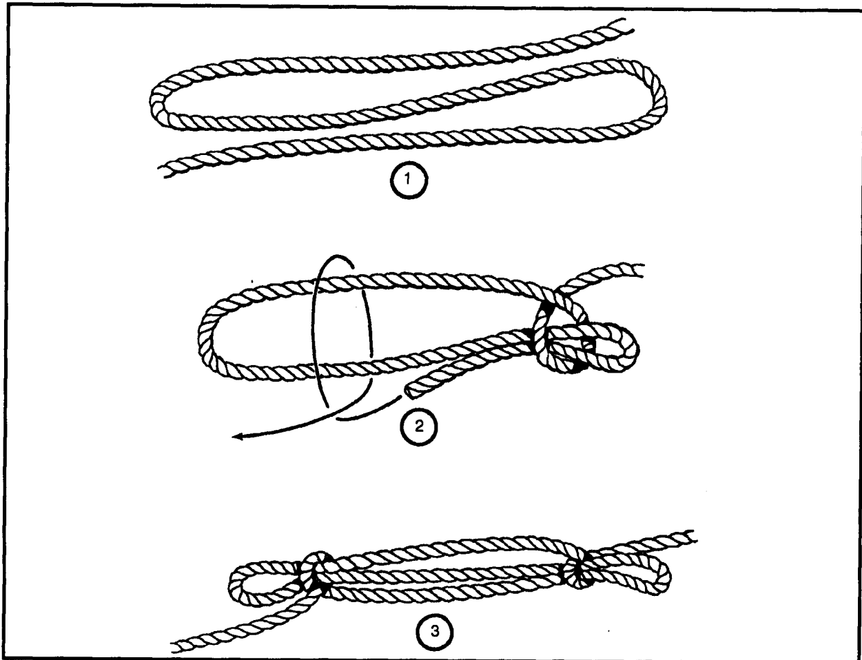
Figure 2-34. Sheepshank
