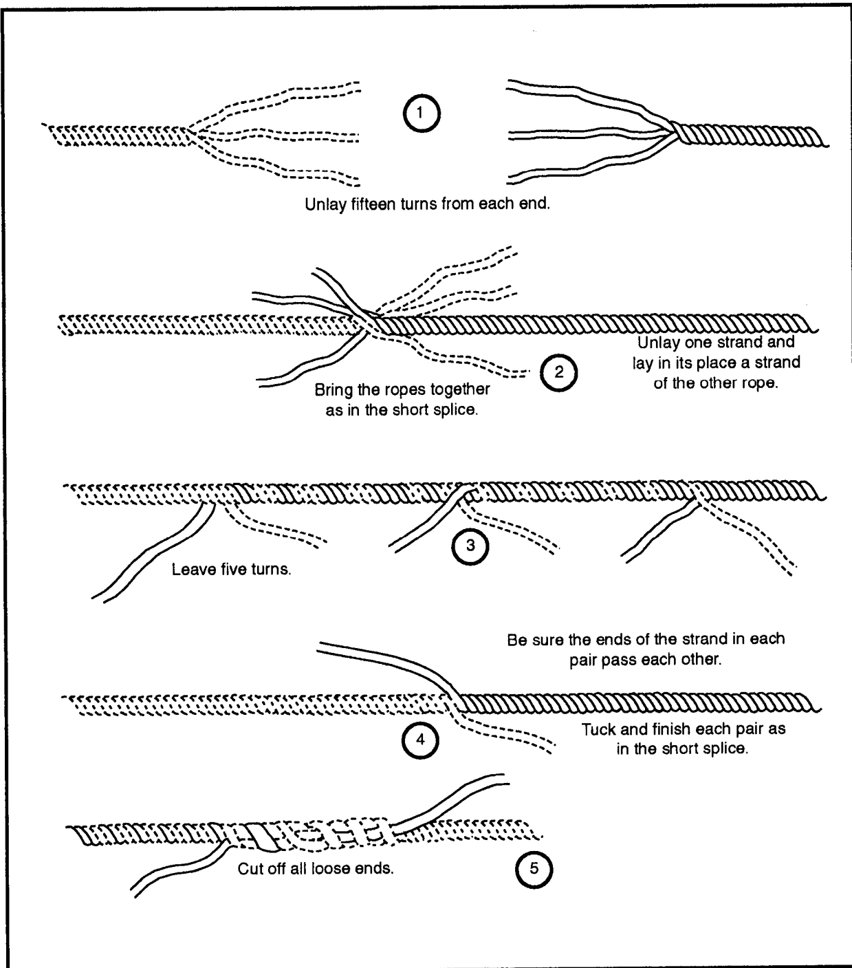
Figure 2-42. Long splice for fiber rope
