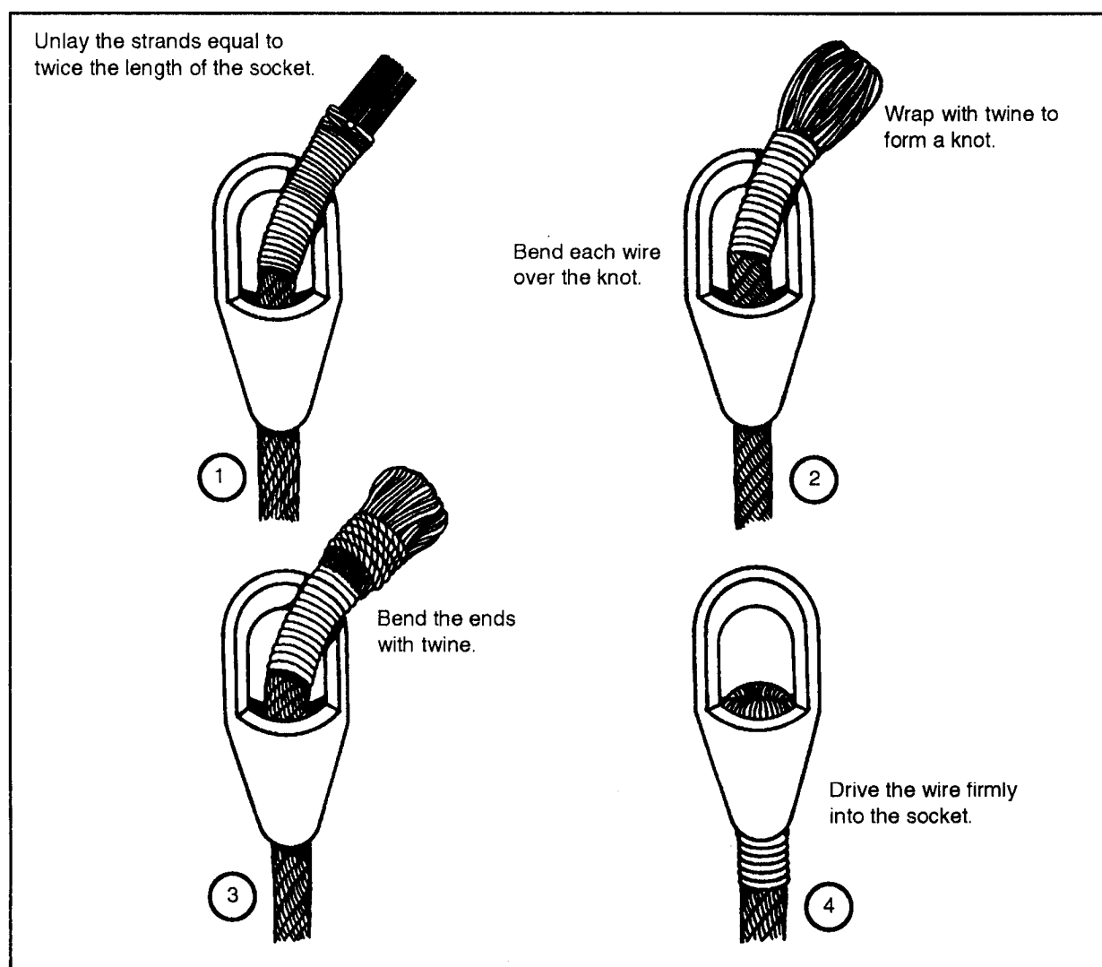
Figure 2-55. Attaching basket sockets by the dry method
