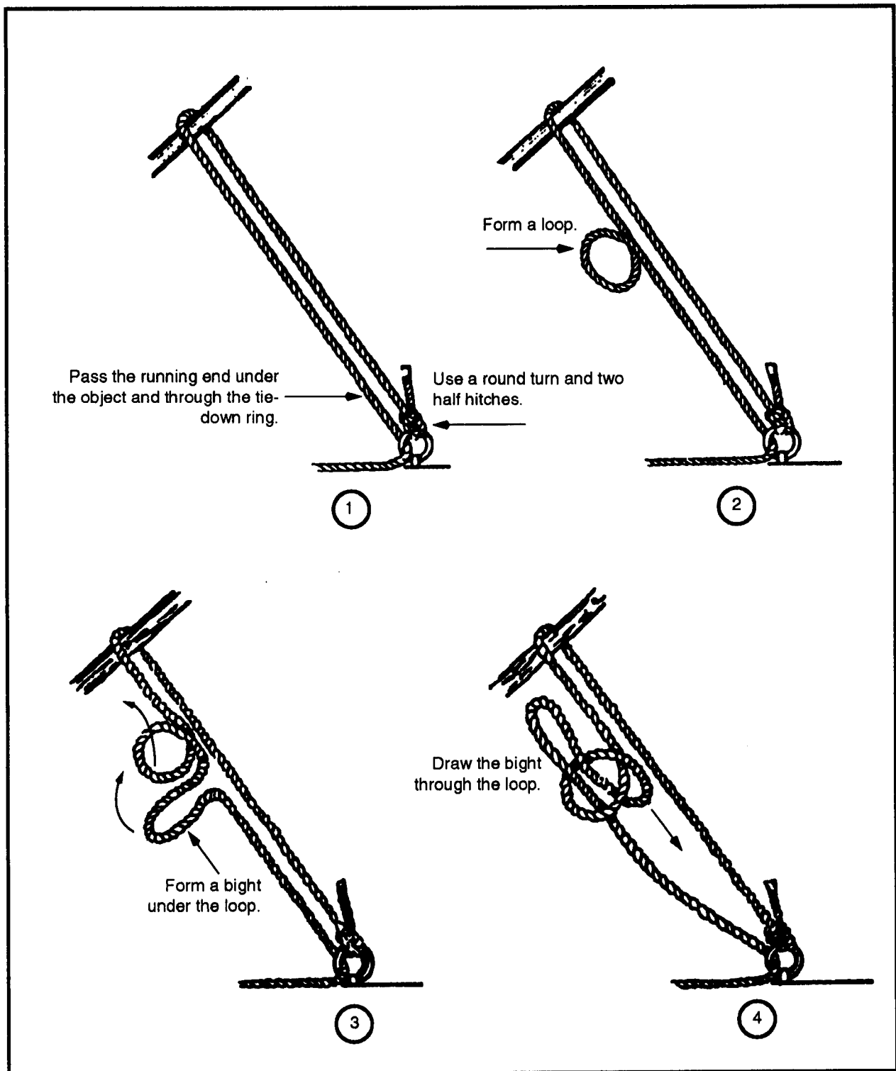
Figure 2-21. Baker bowline
